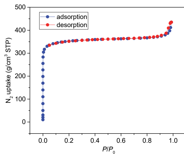
Figure S14. Nitrogen isotherm of CAU-1 (particle size 250 nm) at 77 K. Blue and red symbols represent adsorption and desorption branches, respectively. Points are connected to provide a clear shape of the isotherm.
