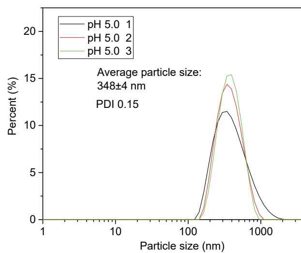
Figure S38. DLS size distribution of CAU-1 nanoparticles in water at pH 5.0, the test was repeated three times.
