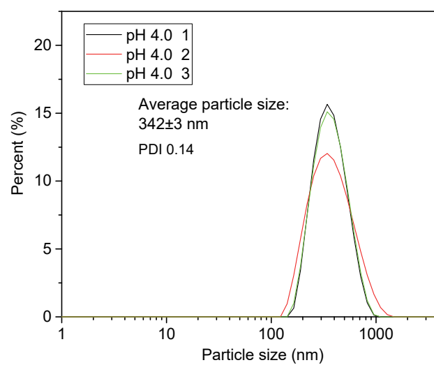
Figure S39. DLS size distribution of CAU-1 nanoparticles in water at pH 4.0, the test was repeated three times.
