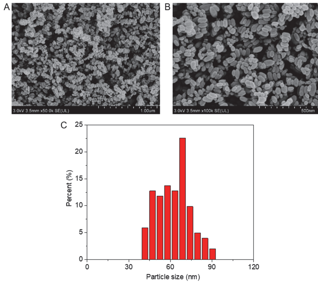
Figure S1. (A) and (B) SEM images of CAU-1 nanoparticles at different scales, scale bars 1 \mu\text{m} and 500 nm, and (C) particle size distribution calculated from SEM images. The average particle size is approximately 60 nm.
