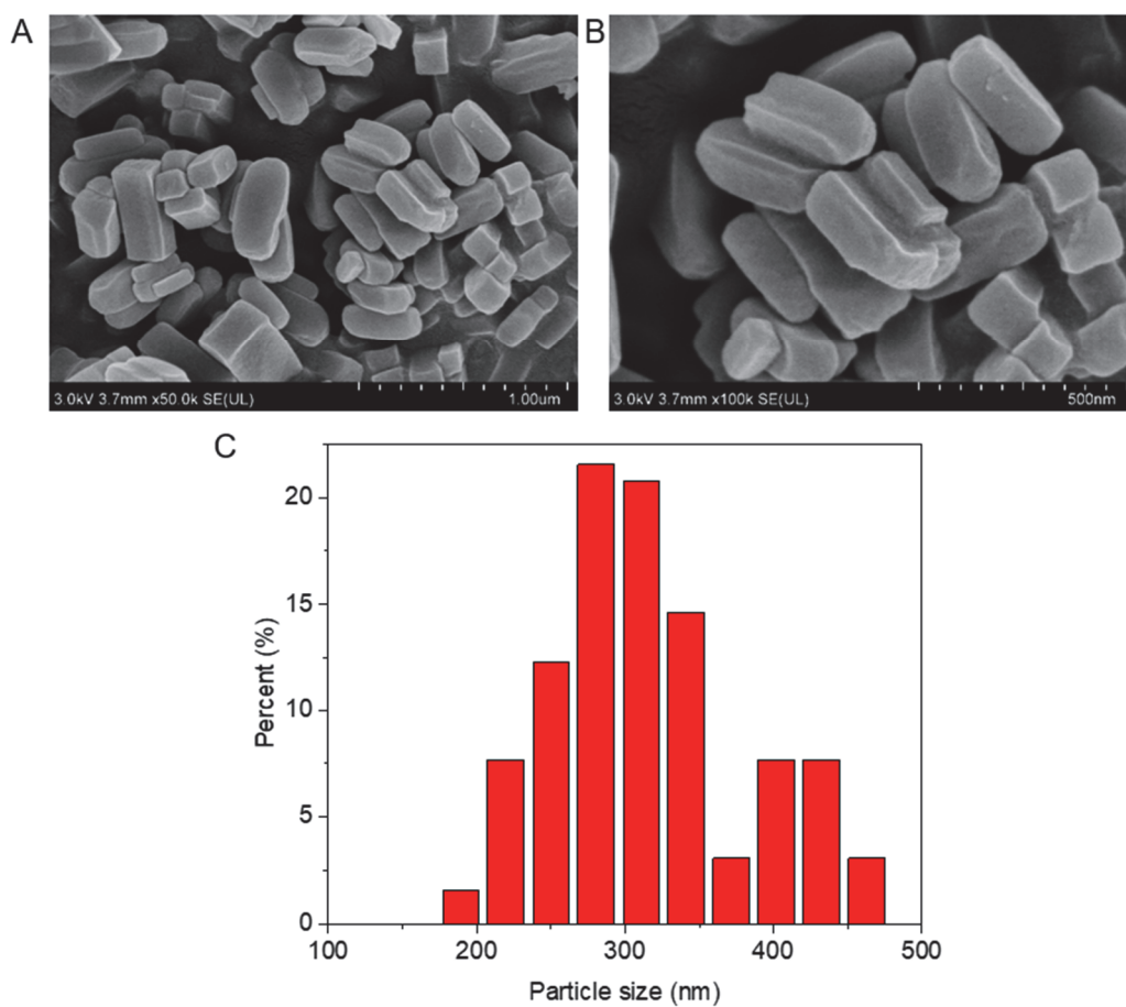
Figure S4. (A) and (B) SEM images of CAU-1 nanoparticles at different scales, scale bars 1 \mu\text{m} and 500 nm, and (C) particle size distribution calculated from SEM images. The average particle size is approximately 320 nm.
