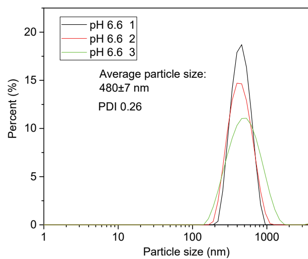
Figure S36. DLS size distribution of CAU-1 nanoparticles in water at pH 6.6, the test was repeated three times.
