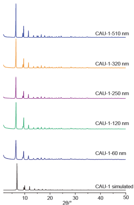
Figure S6. Comparisons of the experimental PXRD pattern of activated CAU-1 in different particle sizes (60, 120, 250, 320, and 510 nm) with the simulated diffraction pattern (black) (Cu K\alpha \lambda = 1.5406 Å).
