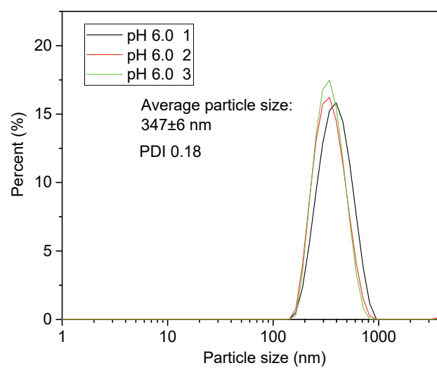
Figure S37. DLS size distribution of CAU-1 nanoparticles in water at pH 6.0, the test was repeated three times.
