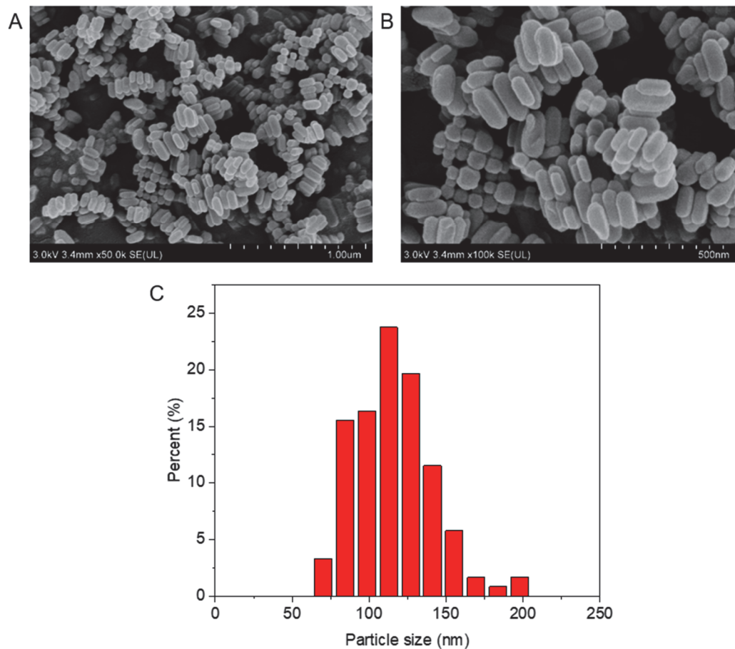
Figure S2. (A) and (B) SEM images of CAU-1 nanoparticles at different scales, scale bars 1 \mu\text{m} and 500 nm, and (C) particle size distribution calculated from SEM images. The average particle size is approximately 120 nm.
