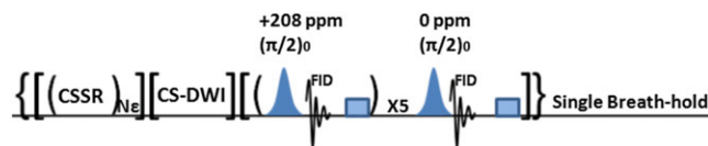
FIGURE 1 The acquisition processes of the proposed method (a total time of 10 s). First, CSSR data were obtained for different delay times with a modified sequence (a total time of 5.3 s). Then, 2D multi-slice DWI data were acquired with the CS method (CS-DWI, a total time of 4.2 s). Finally, spectra were acquired for correction of the flip angle difference between gaseous xenon and dissolved xenon (a total time of 0.4 s). N is the number of different blood-gas exchange delay times \epsilon
